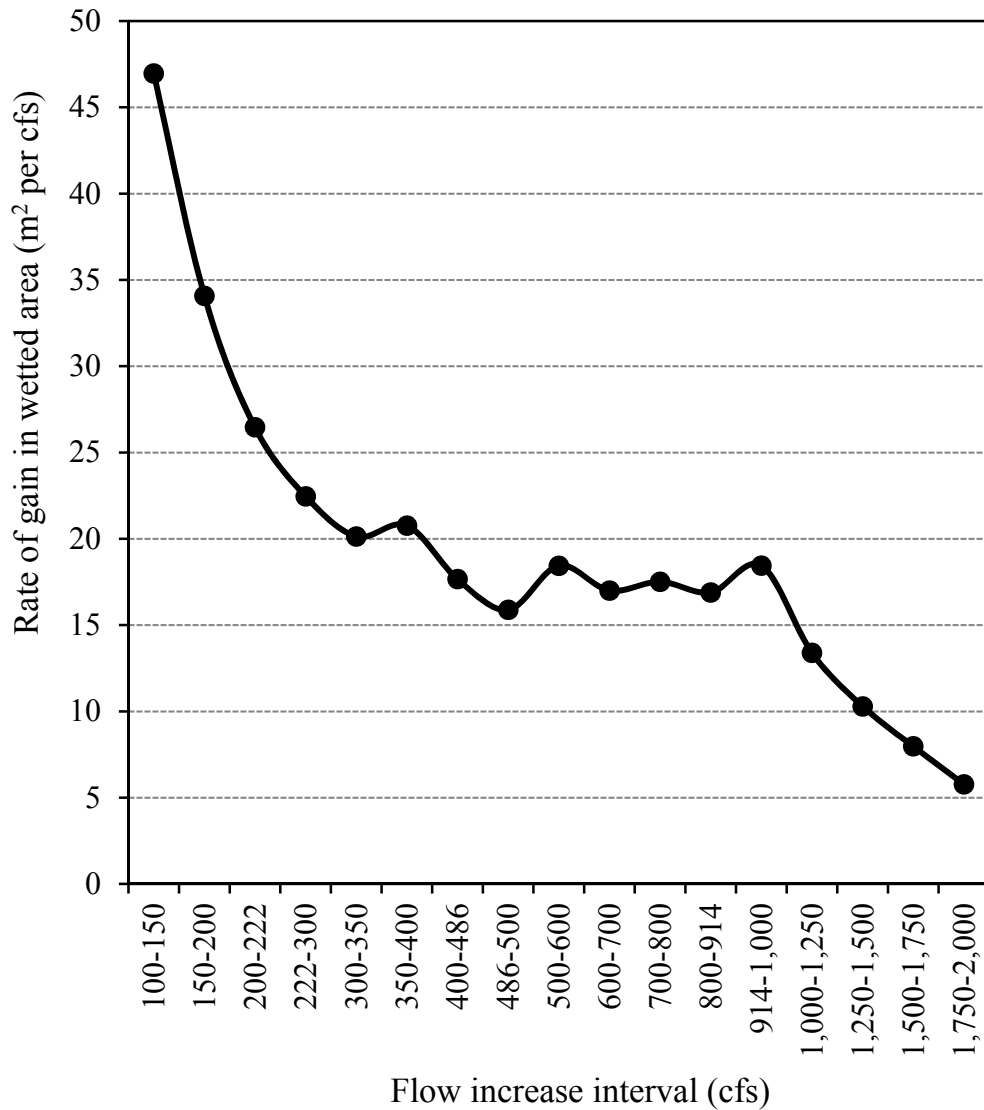
Figure 9. Rate of gain ( \text{m}^2 per cfs) in wetted (inundated) area in the Hawks Nest bypassed reach for progressive flow increases (x-axis) over the range of modeled flows (100 cfs to 2,000 cfs). For example, as flows increase from 100 cfs to 150 cfs (a 50 cfs increase), an additional 2,348 \text{m}^2 of the bypassed reach study area becomes inundated, corresponding to a rate of 47 \text{m}^2 per every 1 unit increase in cfs across this interval (Source: staff).
