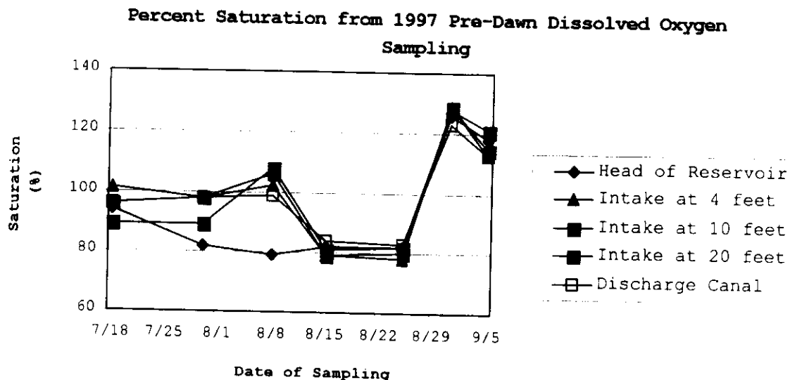
Figure 4. Results of the 1997 dissolved oxygen monitoring at the Weybridge Project (Source: Wallin, 1997a).
